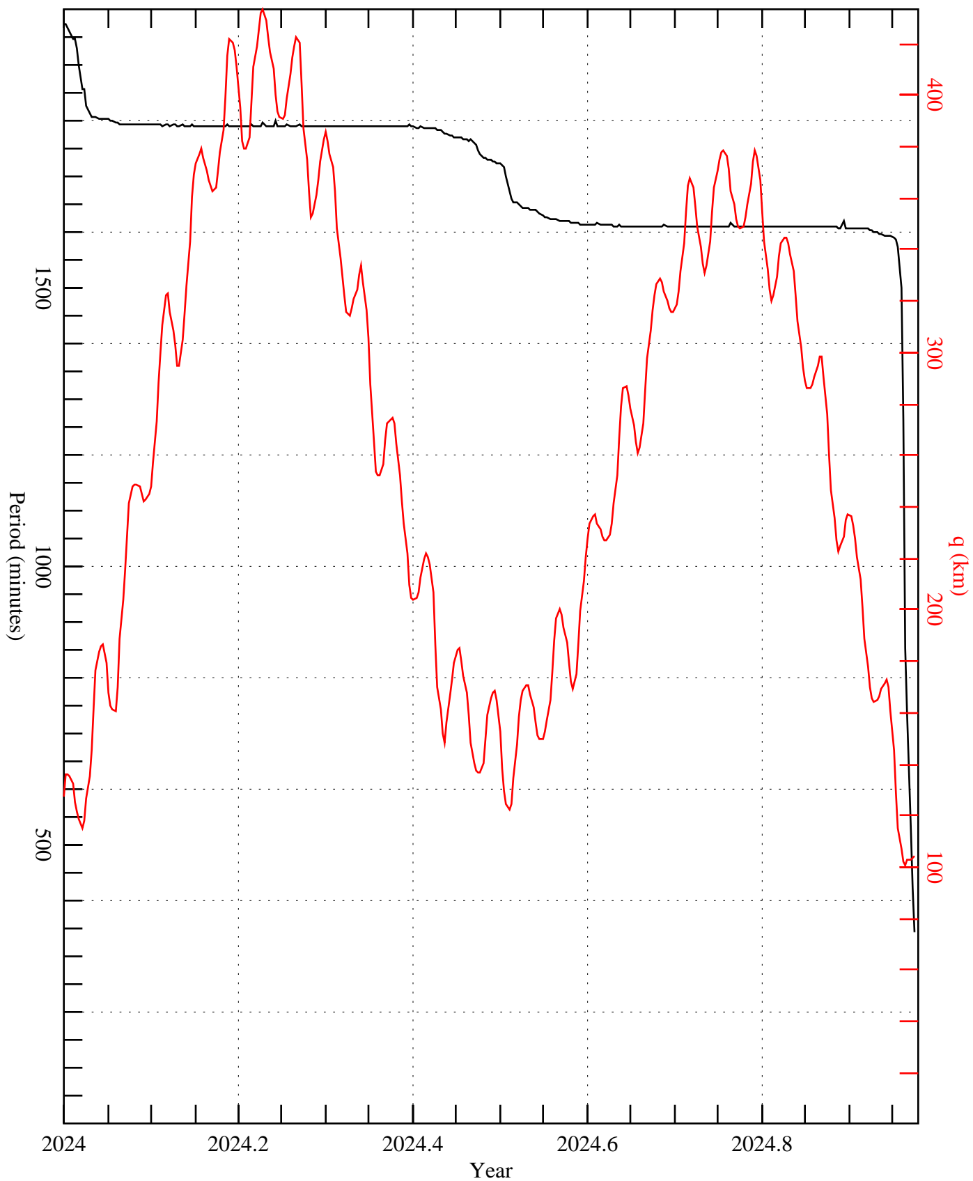
2023-137E = NORAD 57804 = H-2A F47 Stage 2
