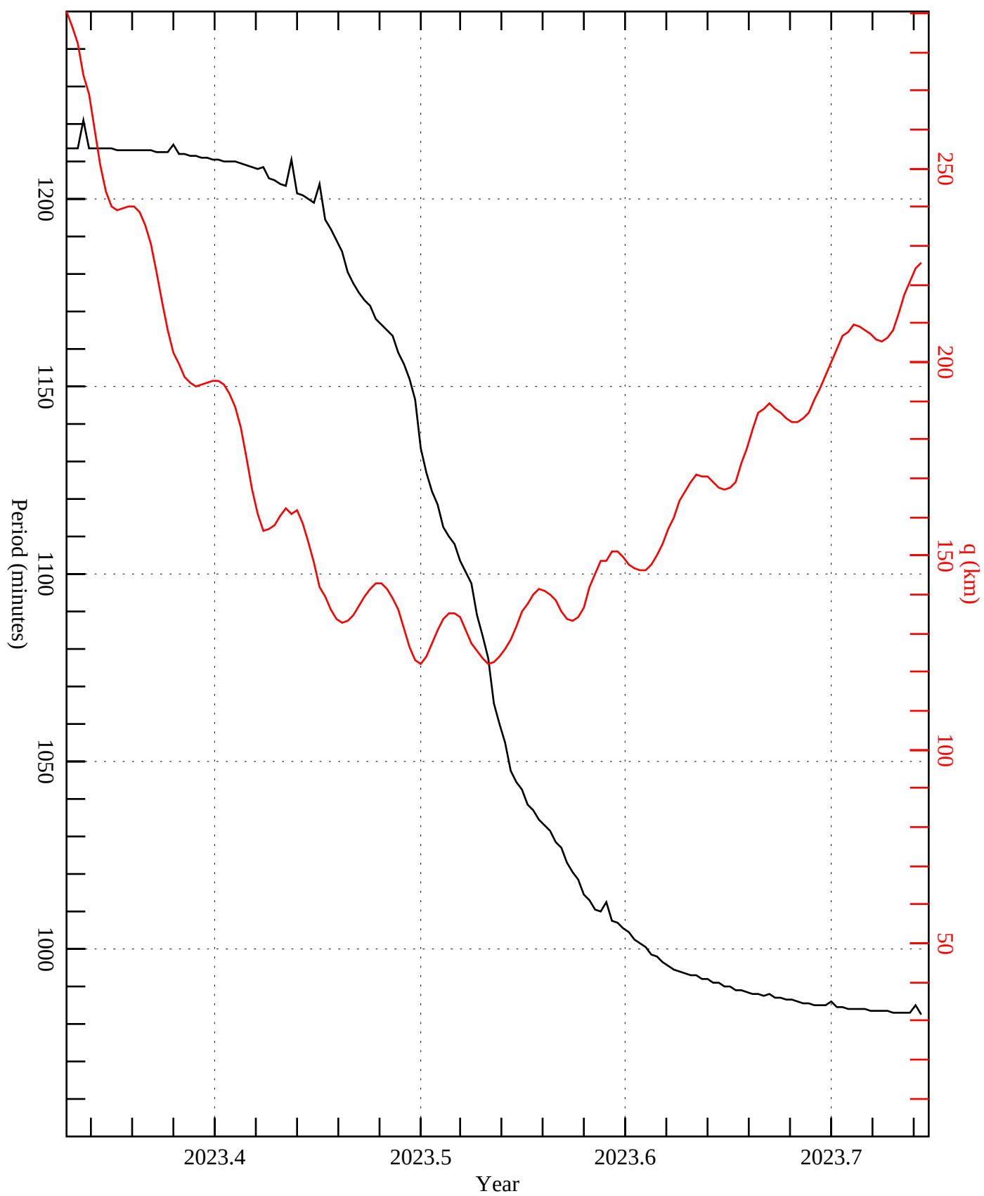
2016-038C = NORAD 41590 = Falcon 9-026 Stage 2
