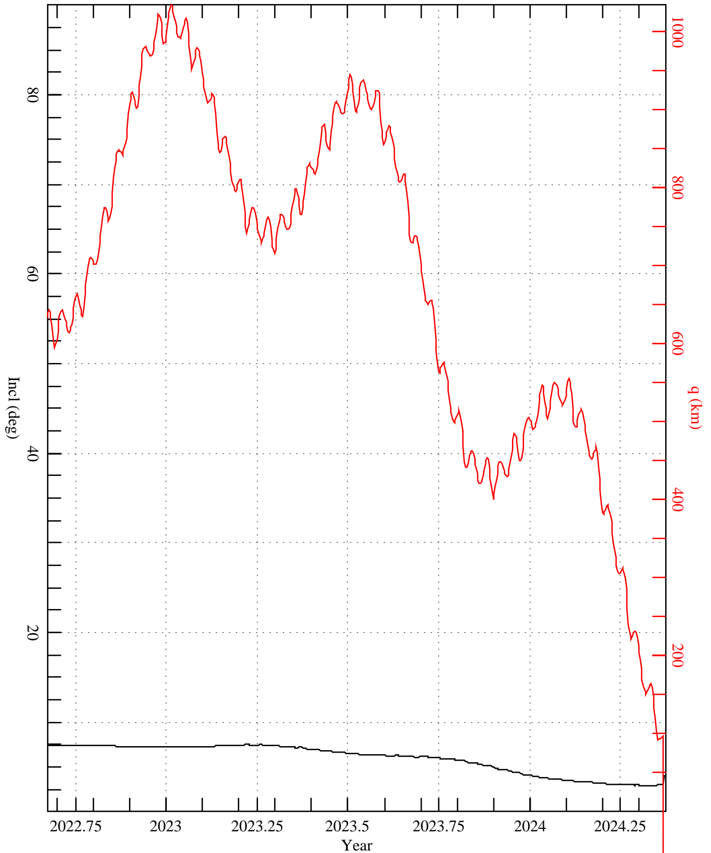
2007-004G = NORAD 30799 = Themis booster
